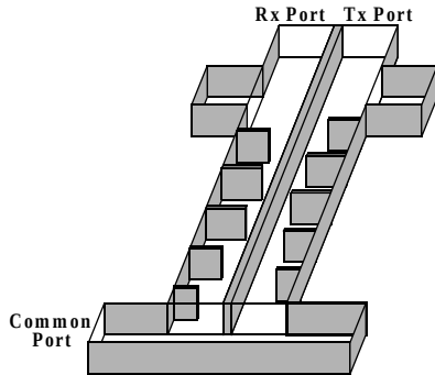
Fig. 7 Principle layout of 18.5 GHz diplexer.
